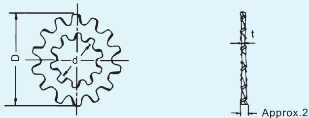
External-Internal type
