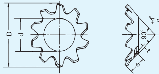
Countersunk type
